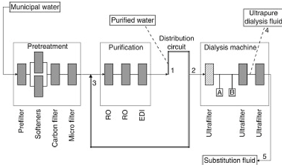
( Fig 2 Diagram for water treatment for substitution fluid delivery )
